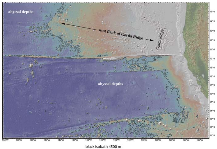
Figure 9-5. GMRT bathymetry of eastern Pacific region of Mendocino Ridge with 4500-m isobath in black. Note the 1 km difference in depth of the seafloor north vs. south of Mendocino Ridge. Abyssal depths (>5000 m) are found immediately south of Mendocino Ridge seafloor depths to the north reflect the young oceanic crust of Gorda Ridge.
