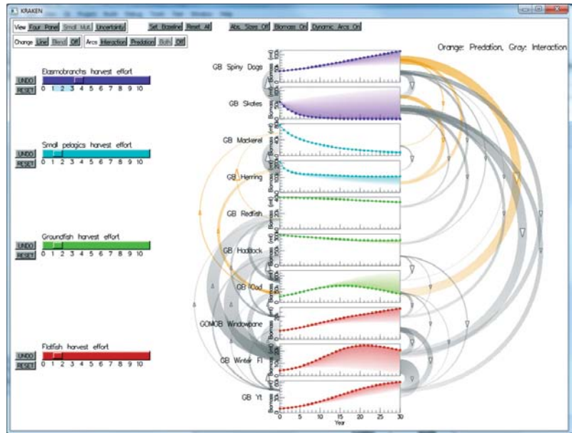
Figure 7-8. Interactive visualization of the forecast for ten Gulf of Maine species based on the NOAA KRAKEN model. The effects of increasing the catch of Elasmobranchs is visualized. The arcs show causal links in the model with predation in yellow and species competition in grey.
