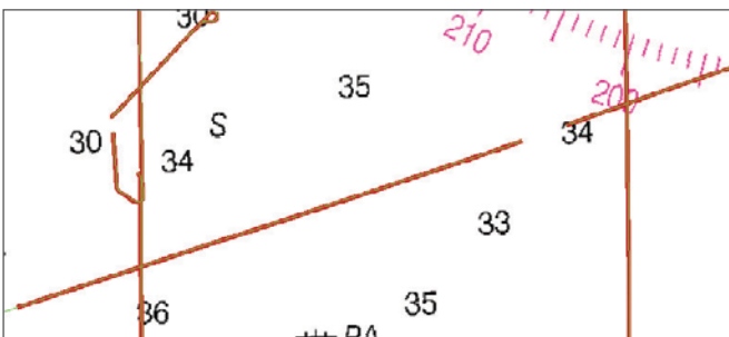
Figure 6-2. Red lines represent track lines run by the Dyson in areas of the Bering Sea where sparse hydrographic data exists, indicated by white space on the chart.
